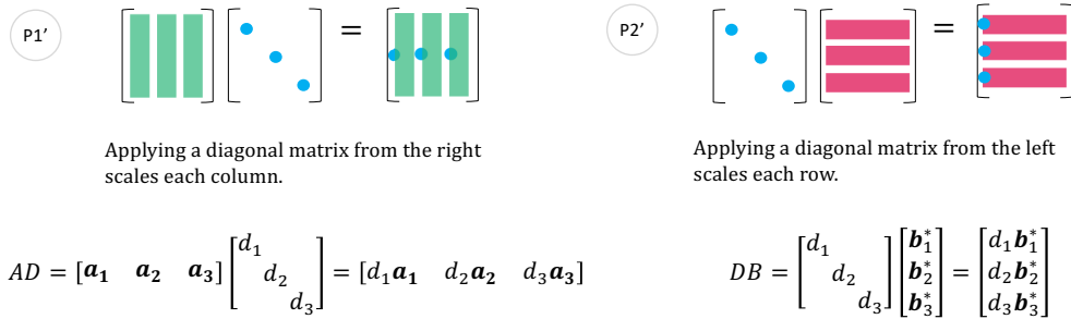
Figure 8: Pattern 1', 2' - (P1'), (P2')
