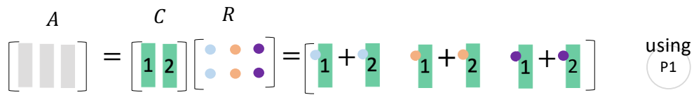
Figure 11: Column Rank in CR
