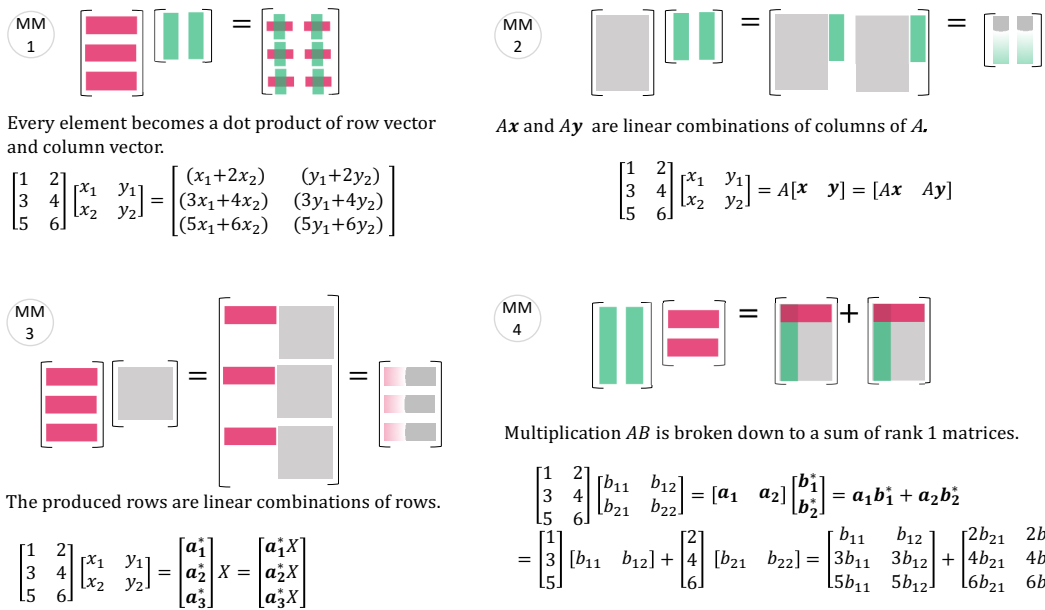
Figure 6: Matrix times Matrix - (MM1), (MM2), (MM3), (MM4)
