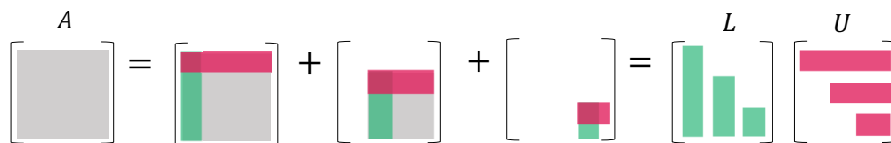
Figure 13: Recursive Rank 1 Matrix Peeling from A
