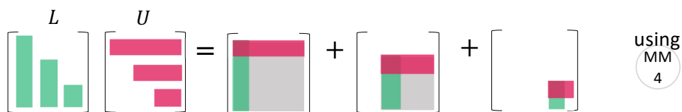
Figure 14: LU rebuilds A
